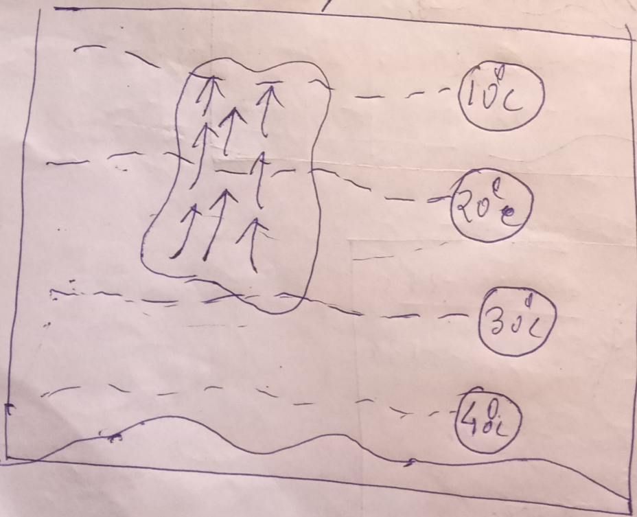
COLLISION-COALSCEANCE TO THEORY OR PRECIPITATION IN LOW LATITUDE AREA
